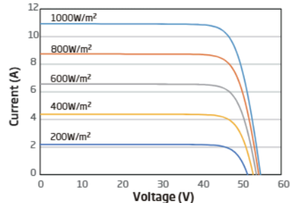
I-V CURVES OF PV MODULE (465W)
